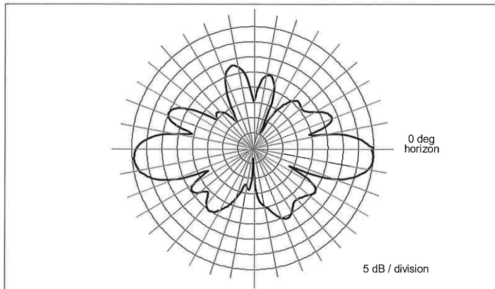
Figure 1. Amphenol 6U4MTSP1X12F70S0– 1900 MHz Vertical-plane Pattern
