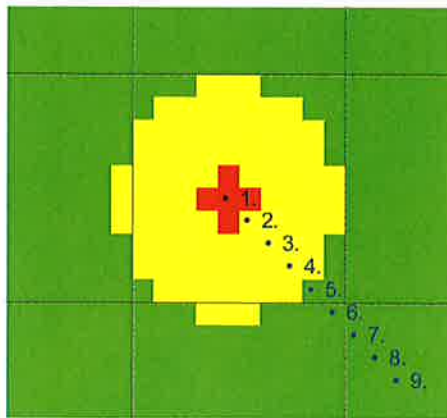
Figure 3. RoofView Graphic Output for Same-height Exposure
